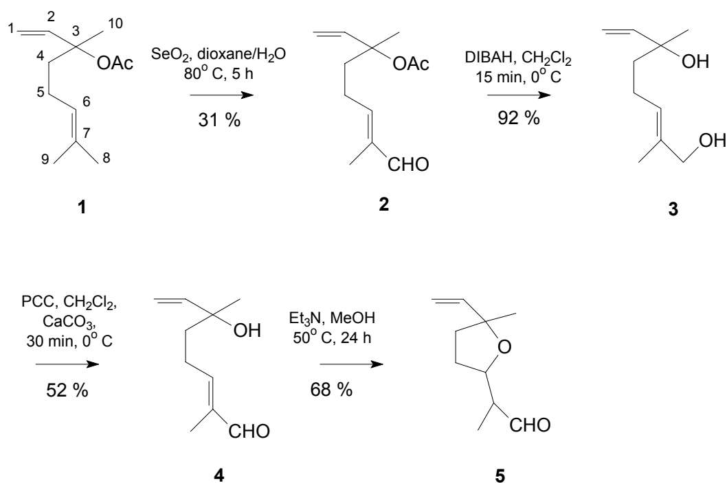
Figure 1: Synthesis of lilac aldehyde isomers
