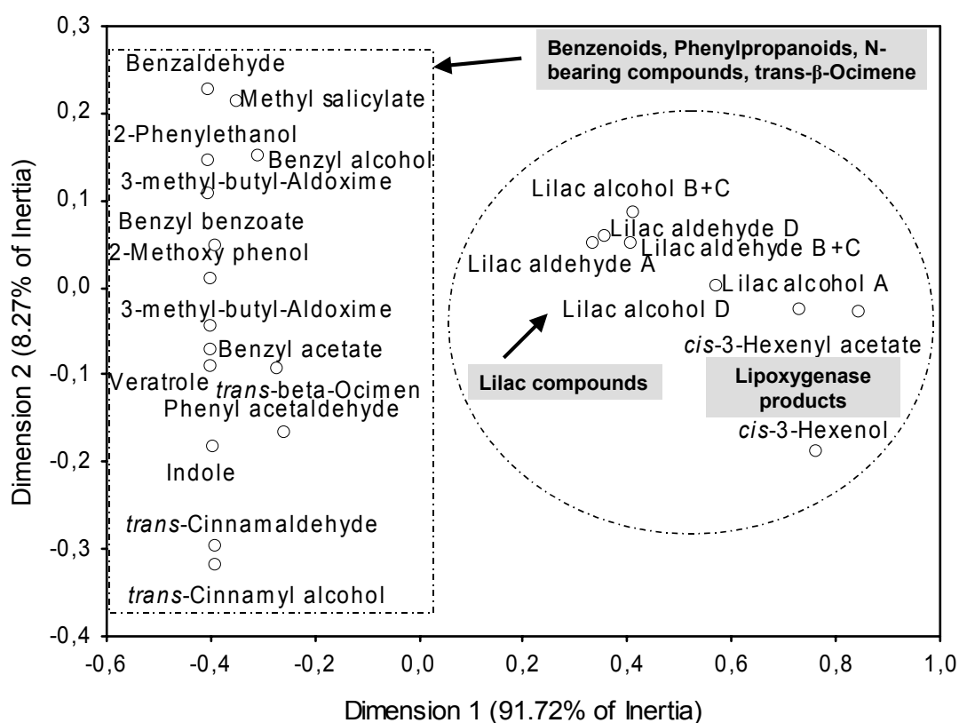
Figure 2: Correspondence analysis of compounds found in male flowers using data of emission patterns of compounds during the preparation process (see Data analyses).
