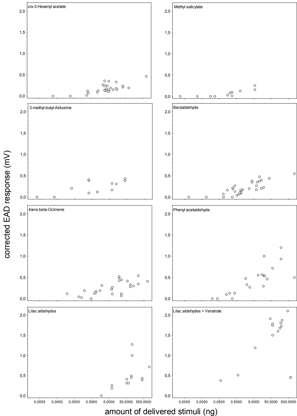
Figure 2: EAD signals of H. bicruris to different amounts of common floral scent compounds of S. latifolia . The EAD response was normalised to a standard stimulus of cis -3-hexenol in a 10^{-3} dilution in paraffine oil (see text).
