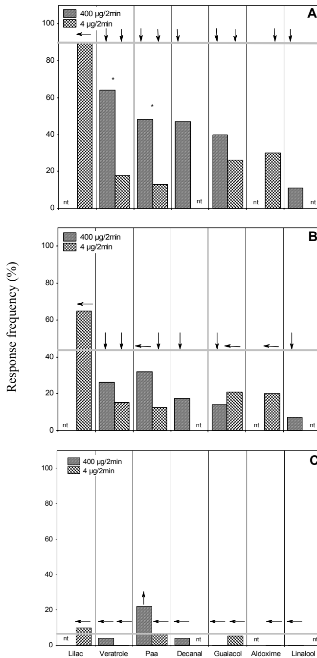
Figure 3: Attractivity of the compounds tested in a wind tunnel. A: orientation flight, B: landing, C: extension of proboscis. — Attractivity of scent of single flowers; ← the tested scent compound is as attractive as the scent of single flowers; ↕ there are significant differences between the tested compound and the scent of single flowers ( \chi^2 -test: p < 0.05 ); *: there are significant differences in attractivity of different doses ( \chi^2 -test: p < 0.05 ); lilac: lilac aldehyde isomers; paa: phenyl acetaldehyde; aldoxime: 3-methyl-butyl-aldoxime; nt: not tested.
