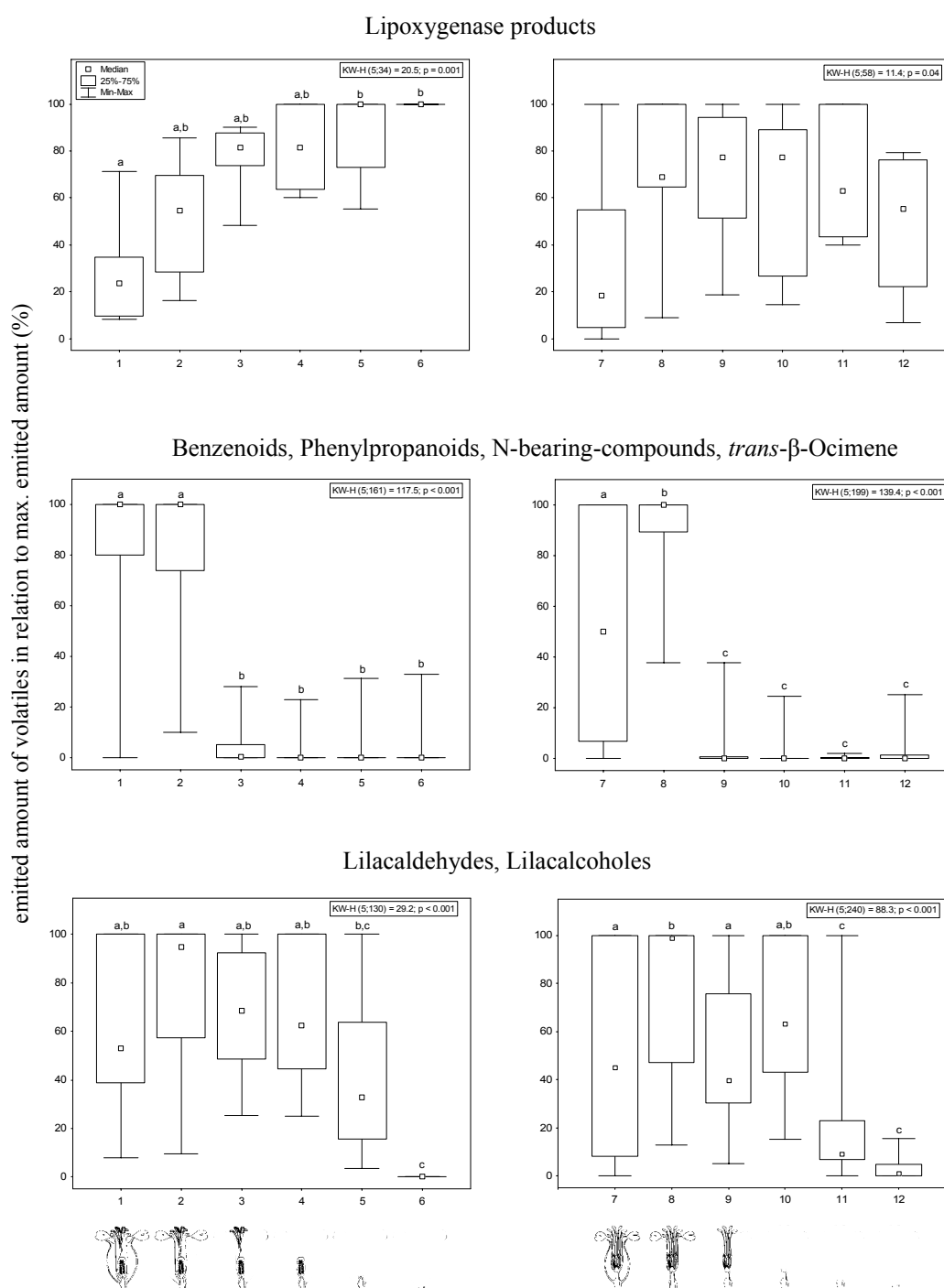
Figure 3: Emission patterns of compound classes in female (left) and male (right) flowers. x-axis: flower and flower preparation stage of females (1-6) and males (7-12) used for collection of volatiles. Volatiles were collected first from whole flowers. Parts of the flowers were then successively removed and volatiles were collected from the remaining “flower” (see Volatile collection).
