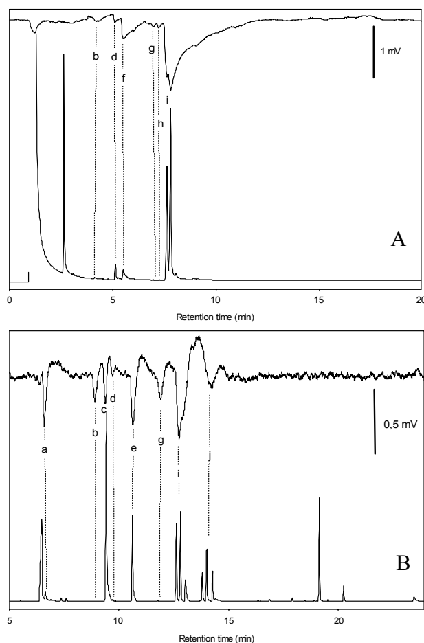
Figure 2: (A) GC-FID/EAD of a S. latifolia extract (number 3 in Table 1) dominated by veratrole and lilac aldehyde isomers, (B) GC-MS/EAD of a S. latifolia extract dominated by \beta -myrcene (number 9 in Table 1). Letters labelling the EAD positive compounds refer to compounds listed in Table 1. Peaks in (A) before retention time of 3min are resulting from the solvent.
